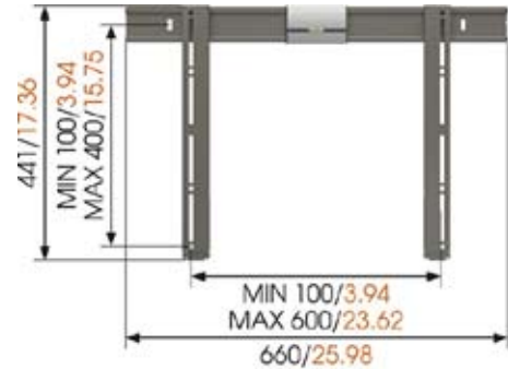
VESA mounting holes mm/inch
