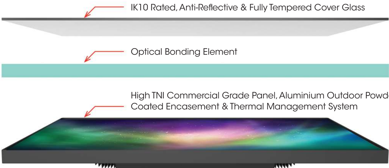
Defining Elements of an Outdoor Commercial Display
